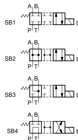
Type SB*: 1 solenoid side B 2 positions (central + external) spring centring
