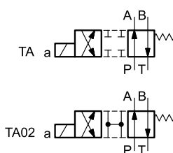
Type TA*: 1 solenoid side A 2 external positions with return spring
