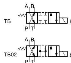
Type TB*: 1 solenoid side B 2 external positions with return spring
