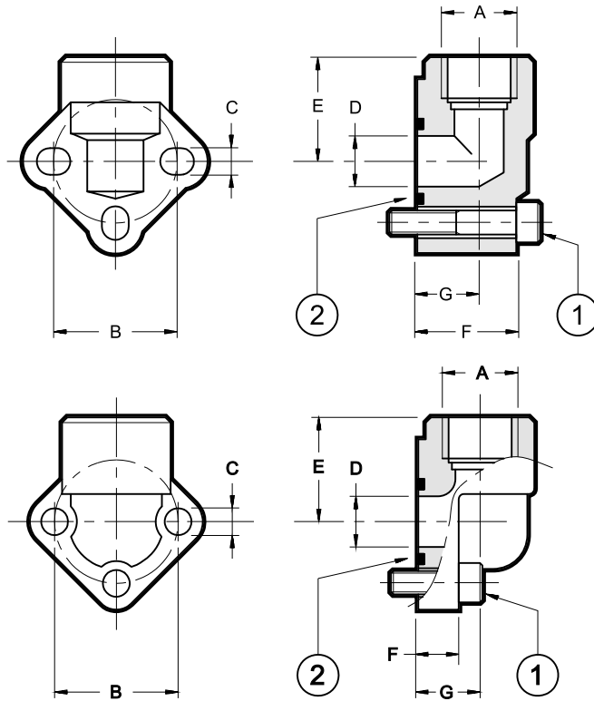
ALUMINIUM FLANGES TYPE RP
